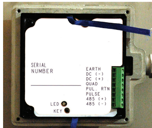
Electronics Module and Connections
